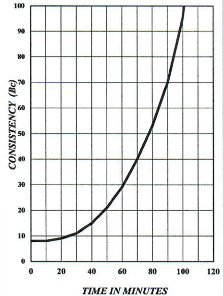
THICKENING TIME TEST API SCHEDULE 5
